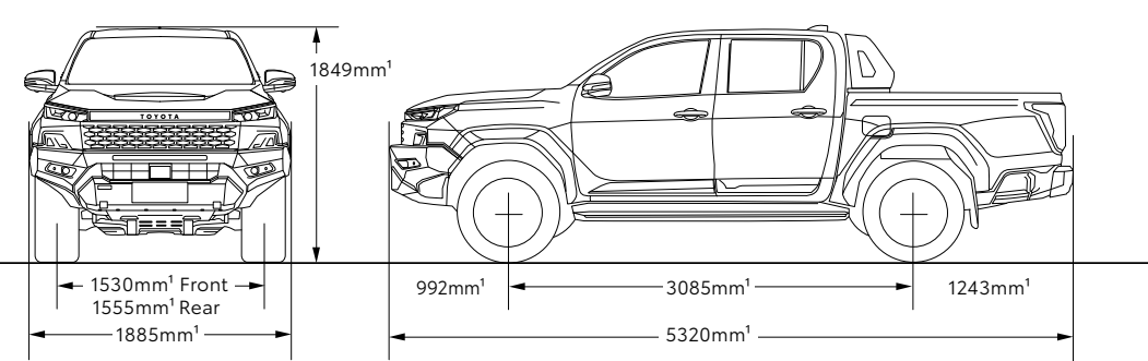
Double-Cab Pick-Up HiLux Rugged X
