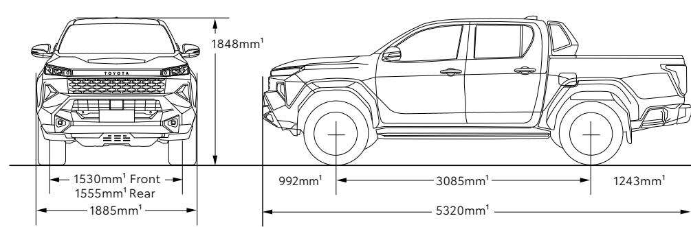
Double-Cab Pick-Up HiLux Rogue
